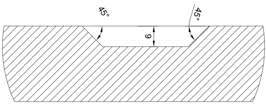
B (1:5)
